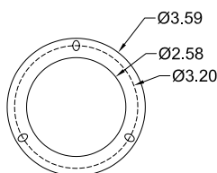
2.5" MOUNTING FLANGE
